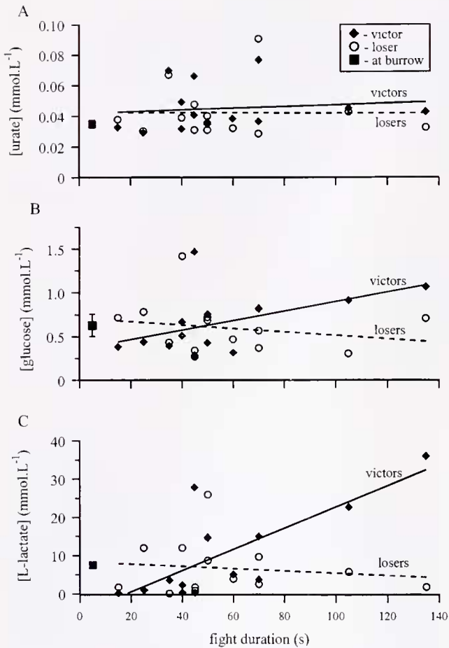
Figure 6. The concentration of (A) uric acid, (B) glucose, and (C) L-lactate ( \text{mmol} \cdot \text{l}^{-1} ) in the hemolymph of male Gecarcoidea natalis guarding burrows during the breeding season (■) and immediately after combat, for losers (○) and victors (◆). Samples were taken from crabs engaged in physical fighting for possession of the burrows, and hemolymph metabolite concentration was plotted against the duration of the fight. The [L-lactate] was statistically dependent on fight duration in the victors but not the losers.
